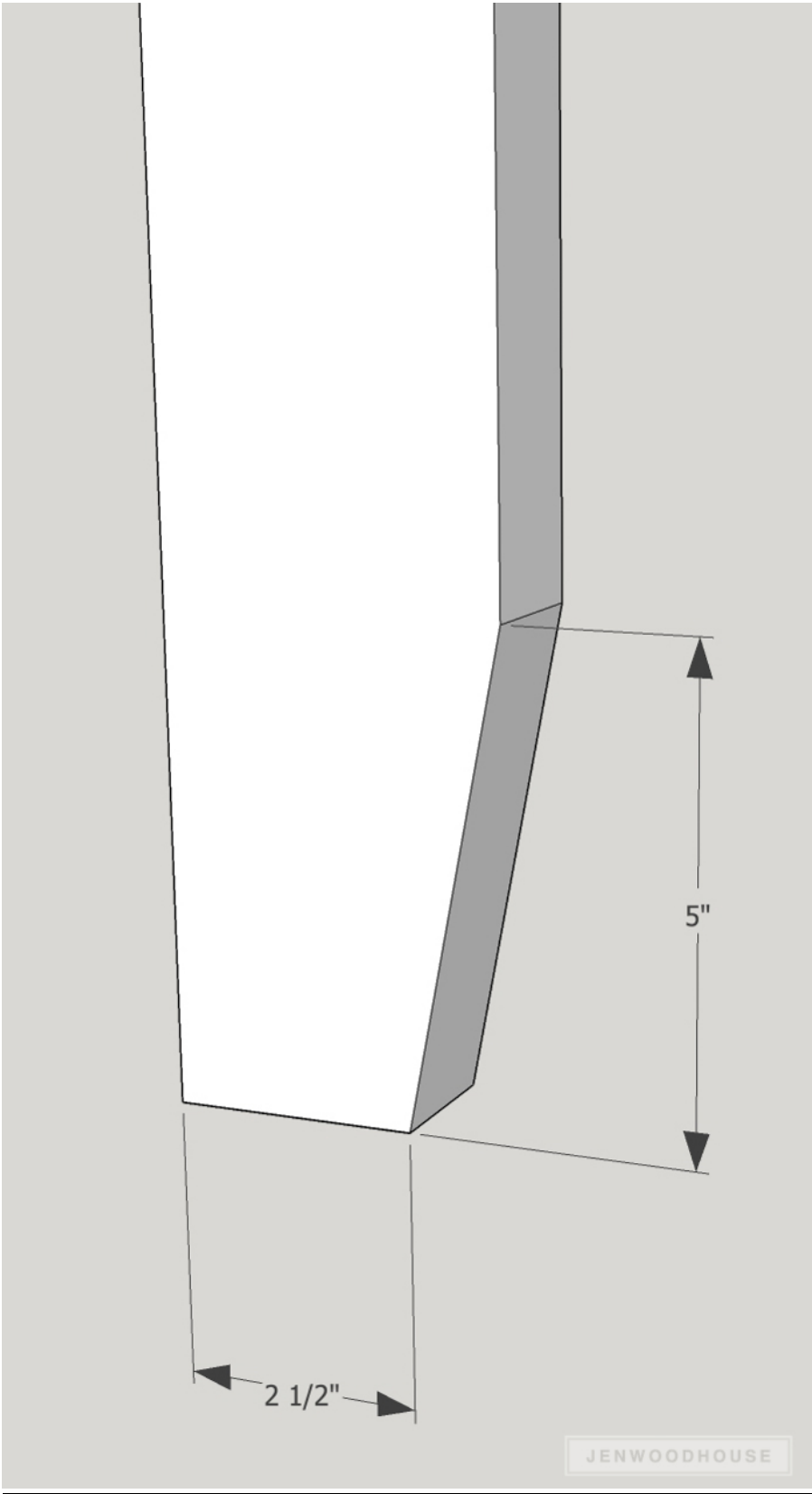
CLOSEUP OF TAPERED FEET
